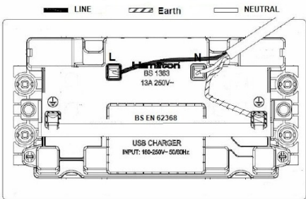
Wiring 13Amp Switched Double Sockets with Twin USB Charging Outlets
