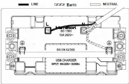
Wiring 13Amp Switched Double Sockets with Twin USB Charging Outlets
