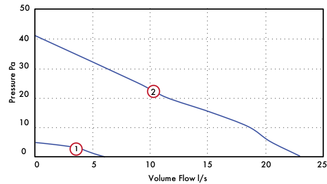
Open Grille
